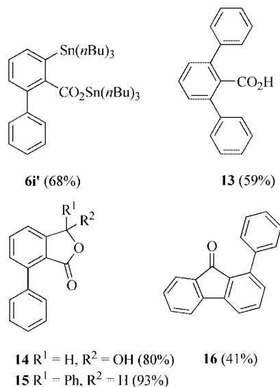
Figure 1. Functionalization of unprotected biphenyl-2-carboxylic acid ( 3 ).
